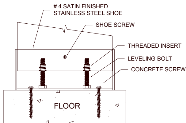
FLOOR MOUNTING DETAIL
