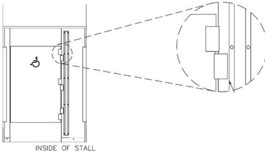
STD. FRONT ELEVATION N T S FOR REFERENCE ONLY
